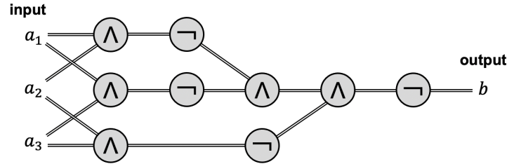
Figure 93: Classical circuit computing the majority value of three bits.
