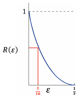
Figure 28: The rate function R(\epsilon) .
