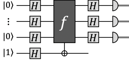
Figure 42: Quantum algorithm for the constant-vs-balanced problem.
