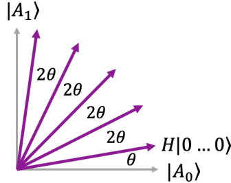
Figure 106: The state |0\dots 0\rangle rotates by angle 2\theta after each iteration.
