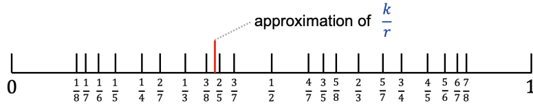
Figure 92: The set of candidates for \frac{k}{r} in the m = 8 case (shown combined).
